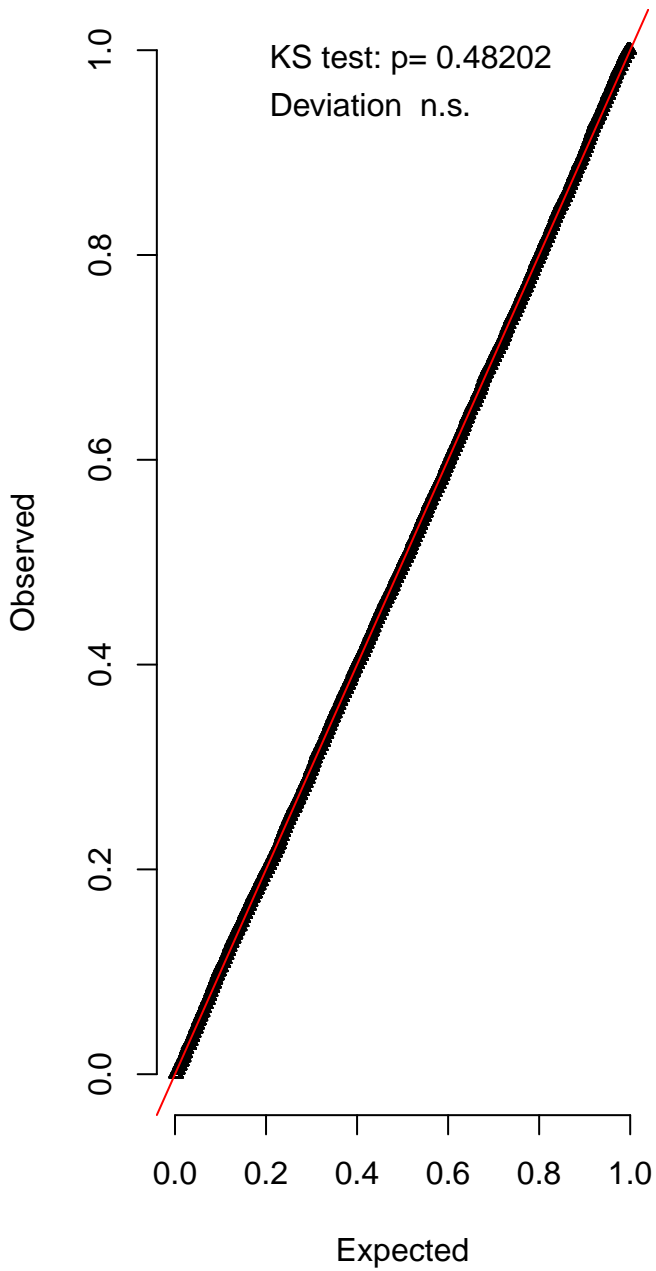
QQ plot residuals
