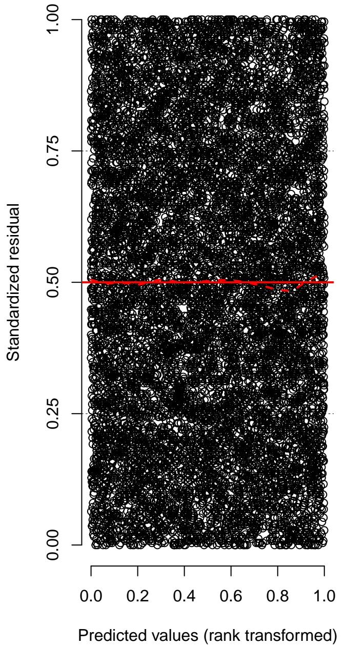
Residual vs. predicted lines should match
