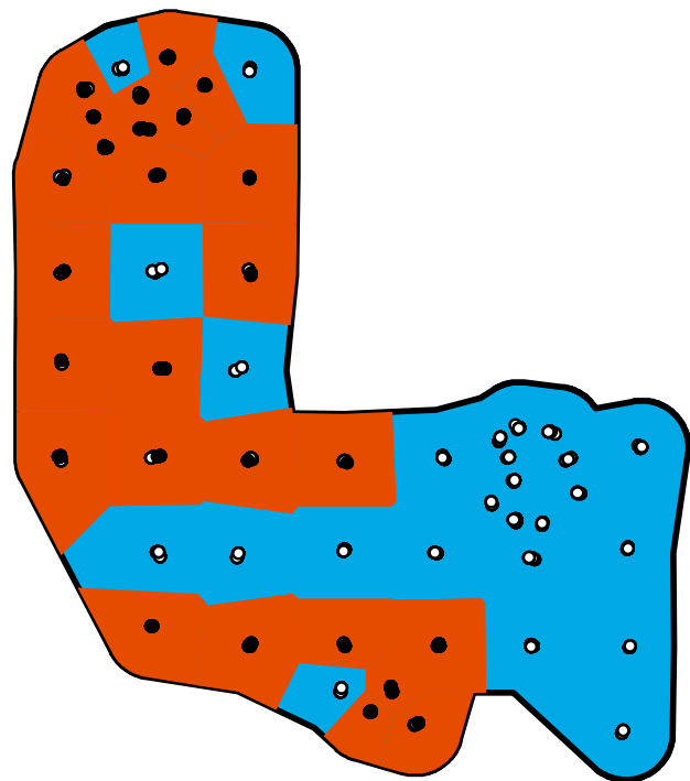
Thiessen Polygons
