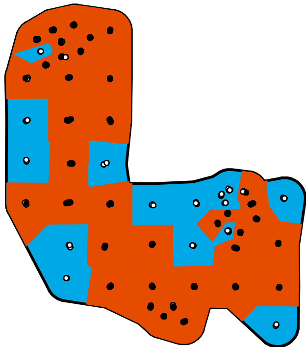
Thiessen Polygons
